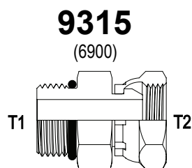
Male ORB / Femelle NPSM Tournant
