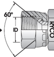
KOMATSU FEMALE & JIS 30° FLARE TYPE MU
