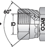
JIS PARALLEL FEMALE SWIVEL & 60° FEMALE SEALING CONE
