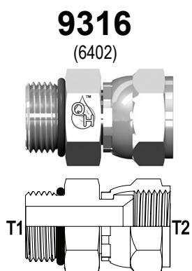
Male ORB / Femelle JIC Tournant
