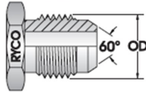
JIS PARALLEL MALE (PF) & 60° MALE SEALING CONE
