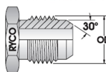
KOMATSU MALE & JIS 30° FLARE TYPE M
